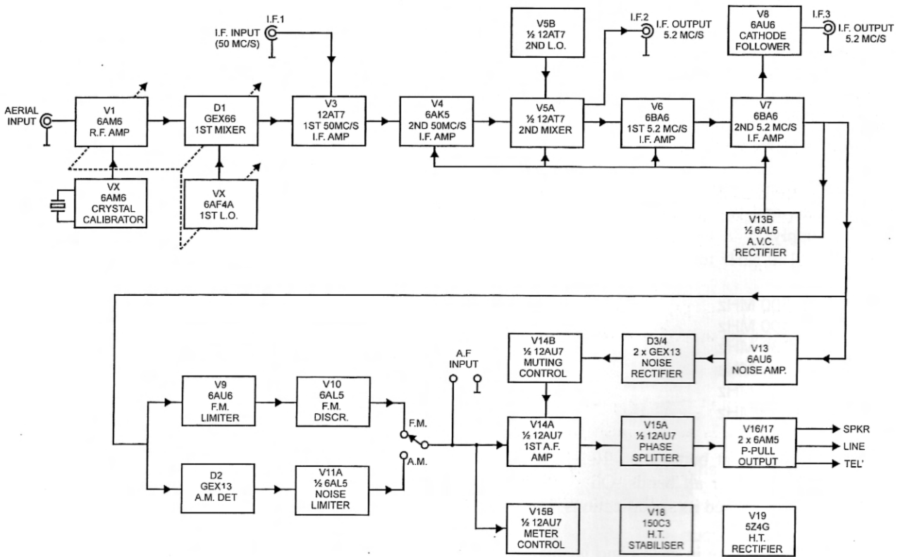
Eddystone 770U MKII Block Diagram
