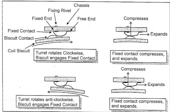
Radial ('TV tuner') contact.
