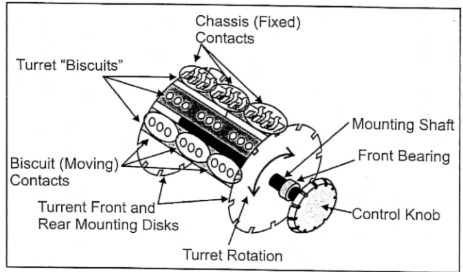
Radial ('TV tuner') simplified construction.
