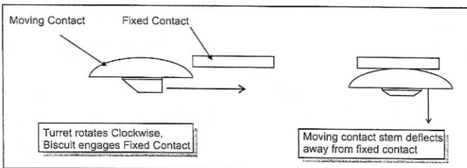
Peripheral (Eddystone 770U) contact.
